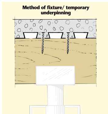
Temporary fixture using wedge-shaped wooden plugs.
